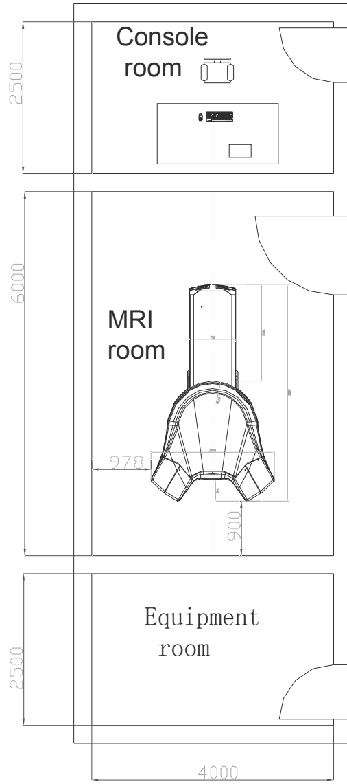
Fig 1: 6 x 4 m Layout
